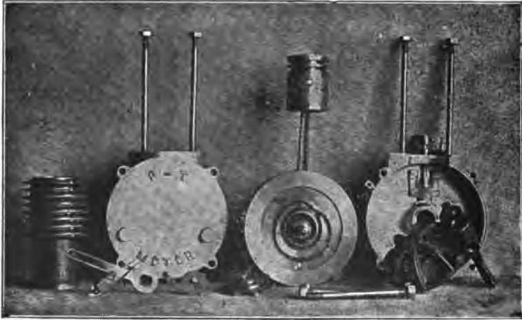
FIG. 237. —The Parts of an Air-Cooled Vehicle Motor, shown for an efficient make of bicycle gasoline engine. The cylinder, carrying radiating ribs, is shown at the left. Next is the outside view of one-half of the crank case; then the trunk piston with the piston rod attached to the crank discs. At the right of the cut is the inside view of the other half of the crank case, with the cylinder head lying in front of it. The crank disc, or fly wheel, shows the double eccentric cam groove for operating the exhaust valve rod, which was a distinctive feature of the earlier Daimler gasoline engines.
